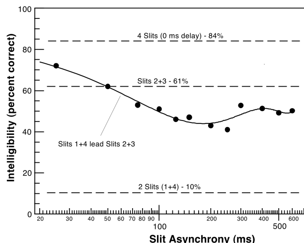
Figure 2. Intelligibility (percent words correct) of sparse spectral sentences containing four narrow-band (1/3 octave) channels as a function of slit asynchrony. Note that intelligibility goes below baseline (slits 2+3) when the slit asynchrony exceeds 50 ms). 27 subjects. Adapted from [19].
